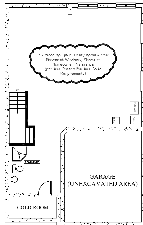
BASEMENT FLOOR PLAN 850 SQ. FT.
