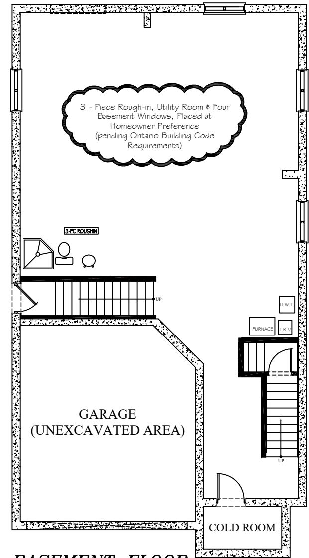
BASEMENT FLOOR PLAN 1,069 SQ. FT.
