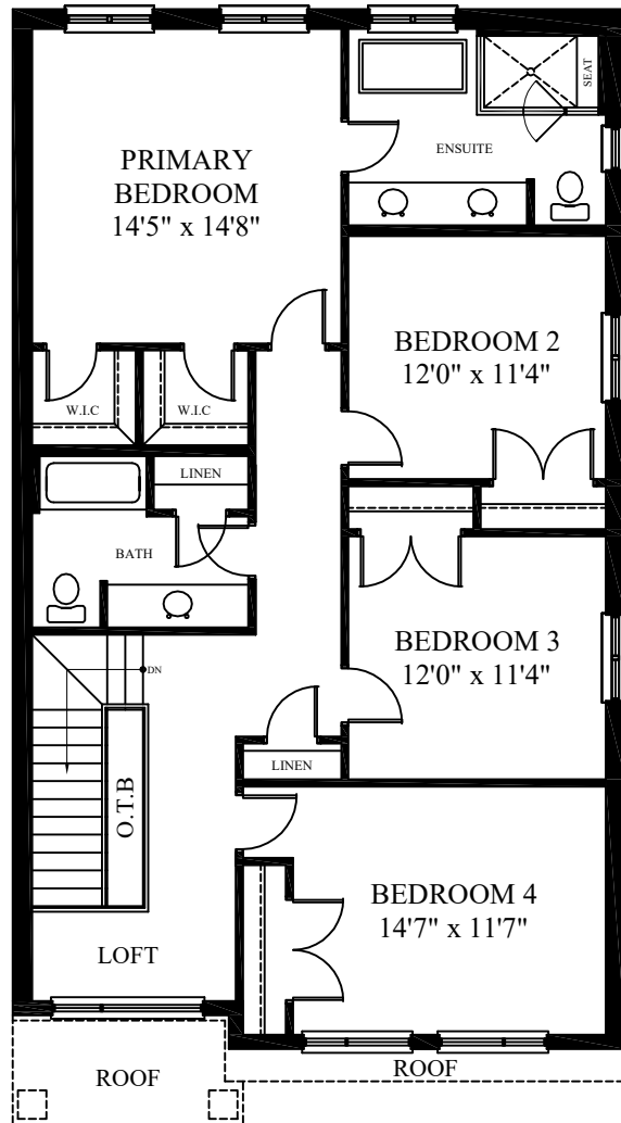
SECOND FLOOR PLAN 1,370 SQ. FT.
