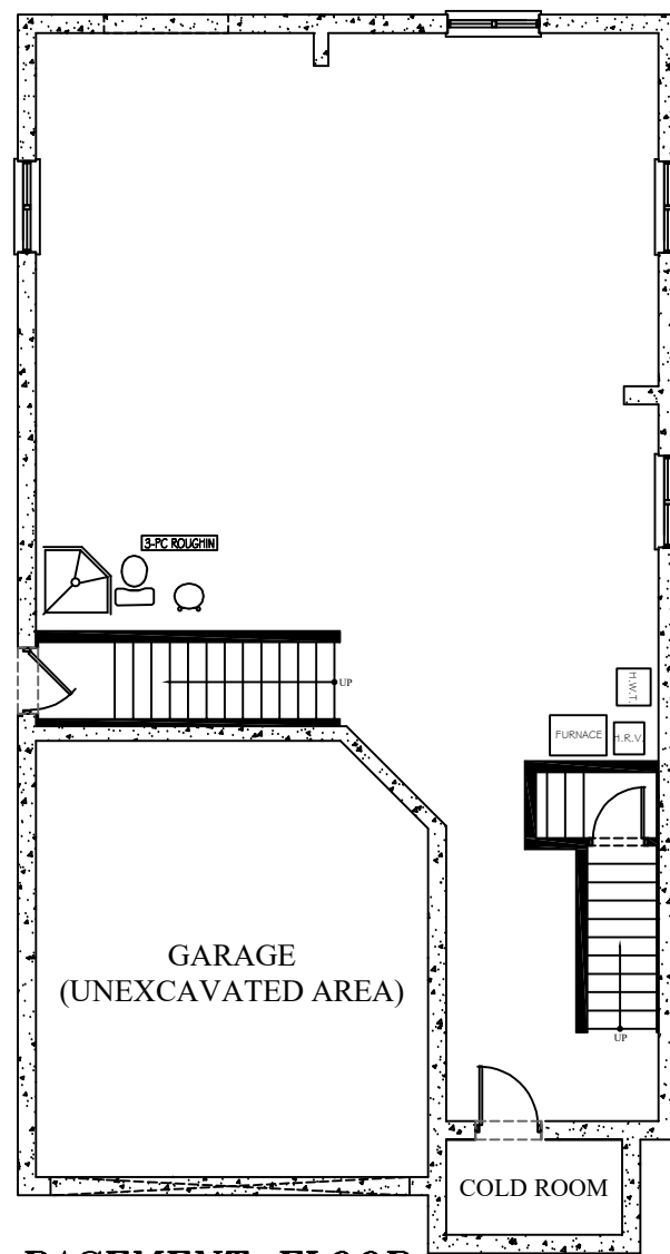
BASEMENT FLOOR PLAN 1,075 SQ. FT.
