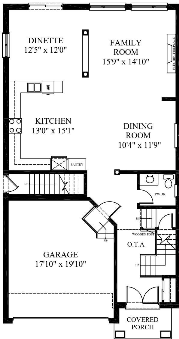
FIRST FLOOR PLAN 1,206 SQ. FT.
