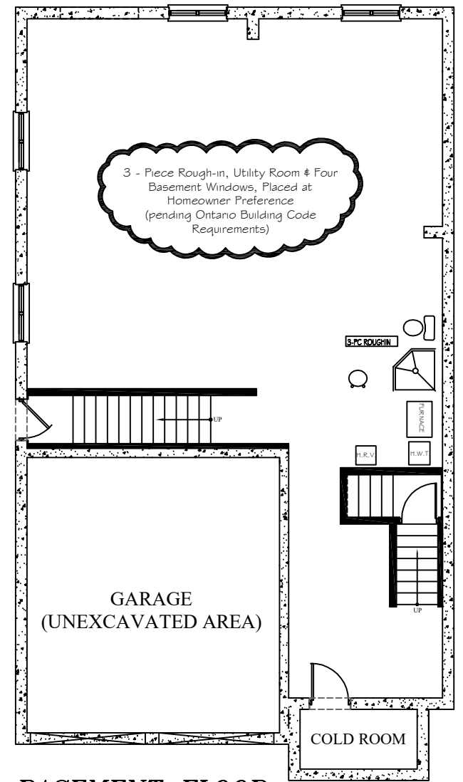
BASEMENT FLOOR PLAN 1,141 SQ. FT.
