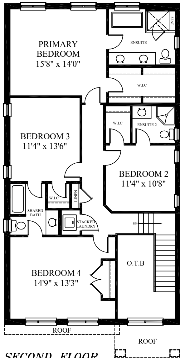
SECOND FLOOR PLAN 1,488 SQ. FT.
