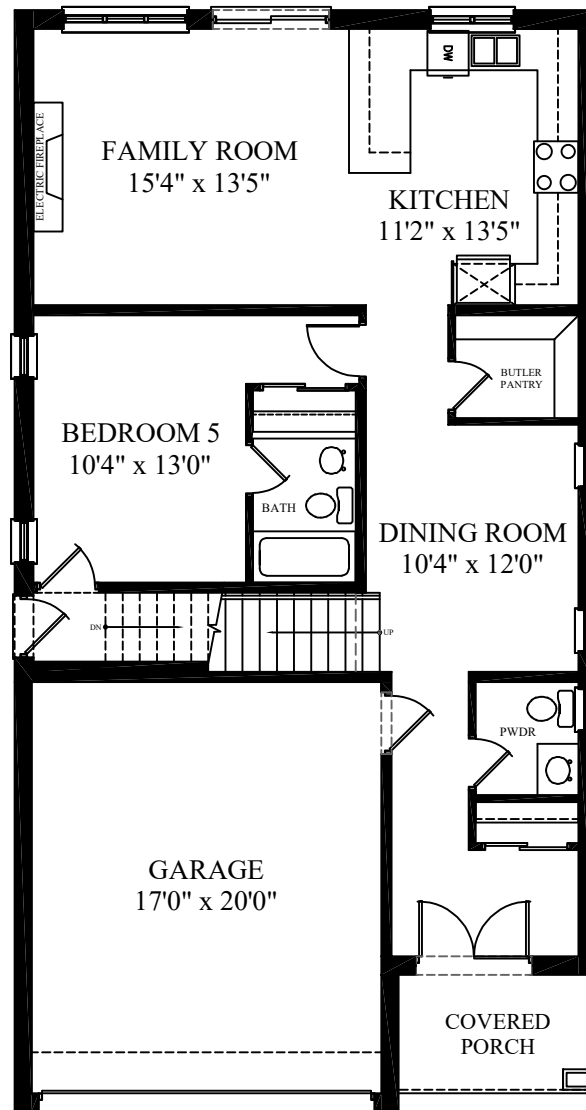
FIRST FLOOR PLAN 1,075 SQ. FT.
