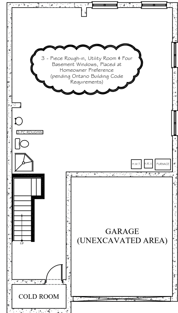
BASEMENT FLOOR PLAN 902 SQ. FT.
