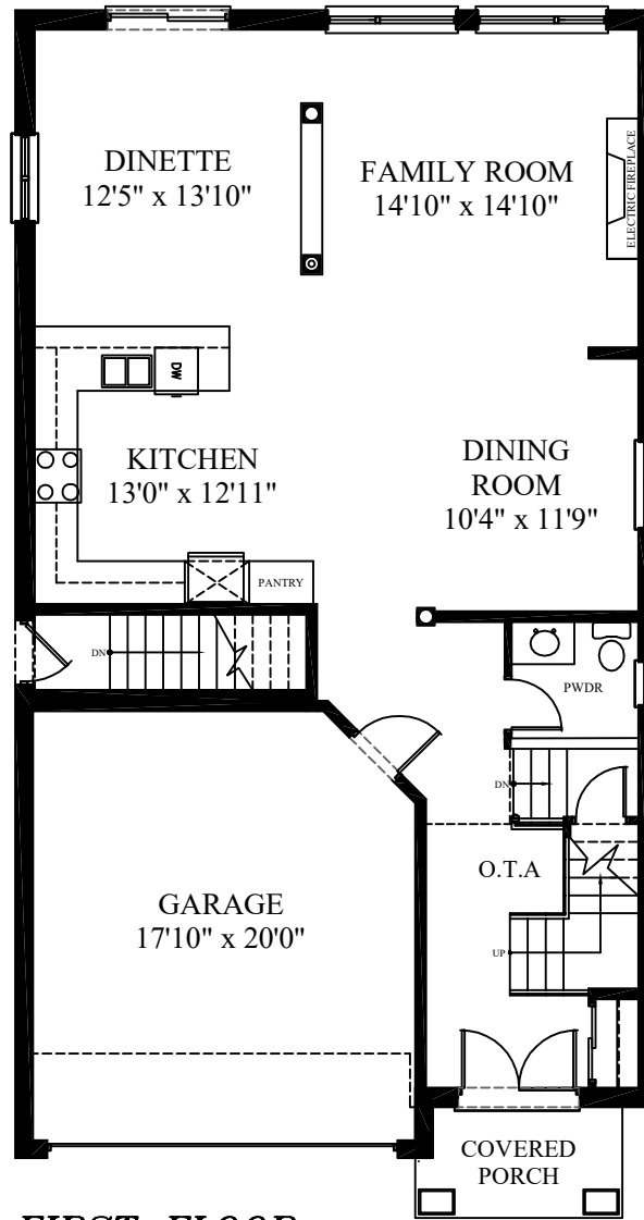
FIRST FLOOR PLAN 1,197 SQ. FT.
