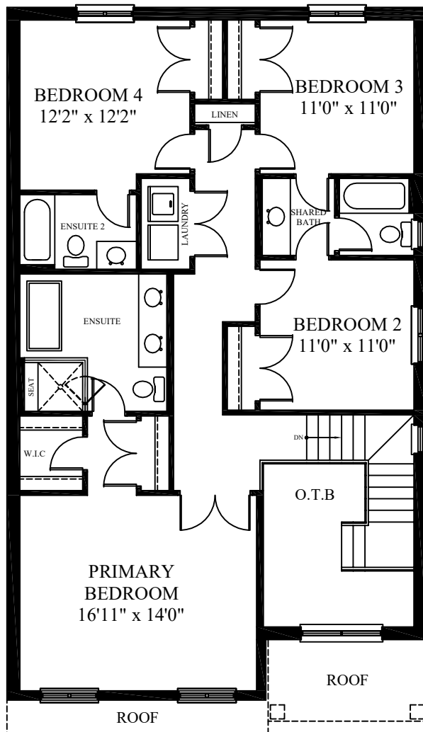
SECOND FLOOR PLAN 1,438 SQ. FT.
