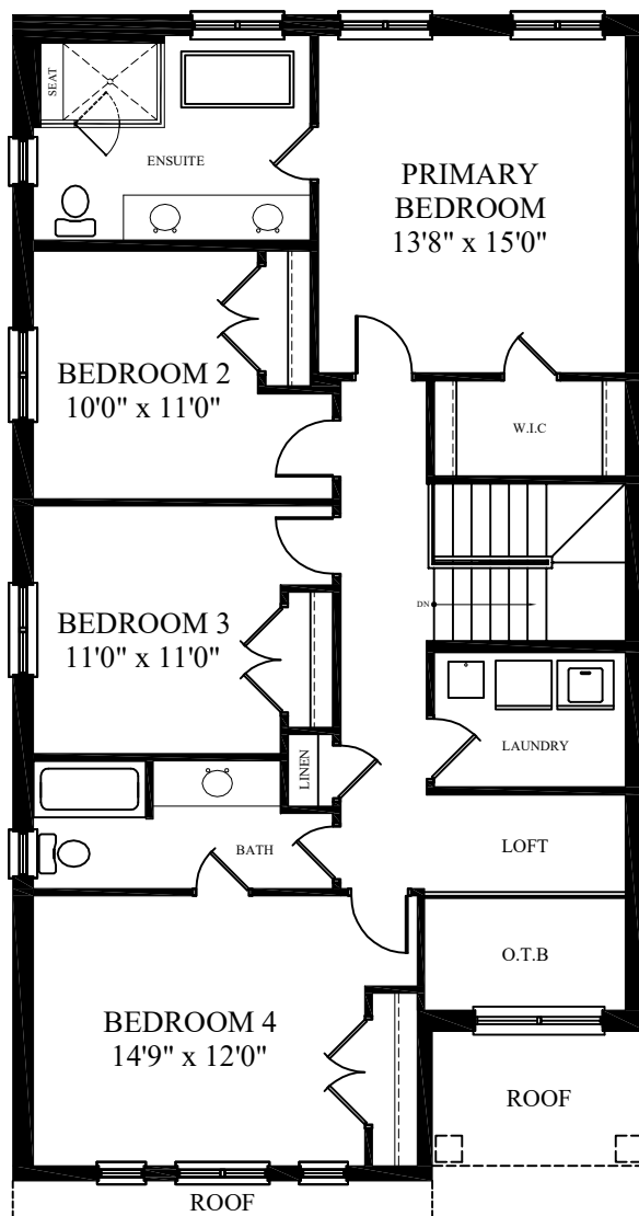
SECOND FLOOR PLAN 1,396 SQ. FT.
