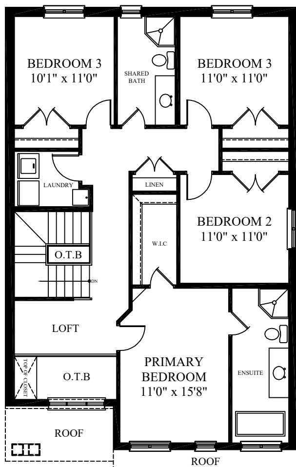
SECOND FLOOR PLAN 1,276 SQ. FT.
