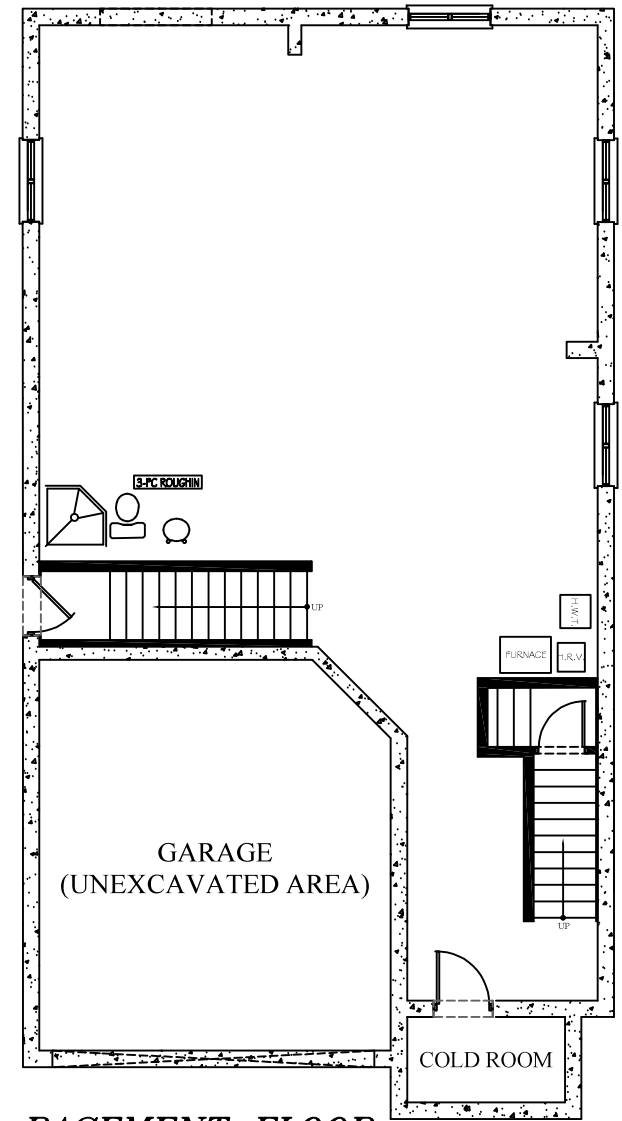
BASEMENT FLOOR PLAN 1,075 SQ. FT.
