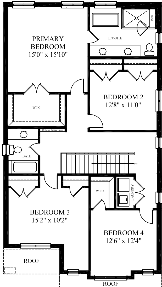
SECOND FLOOR PLAN 1,478 SQ. FT.
