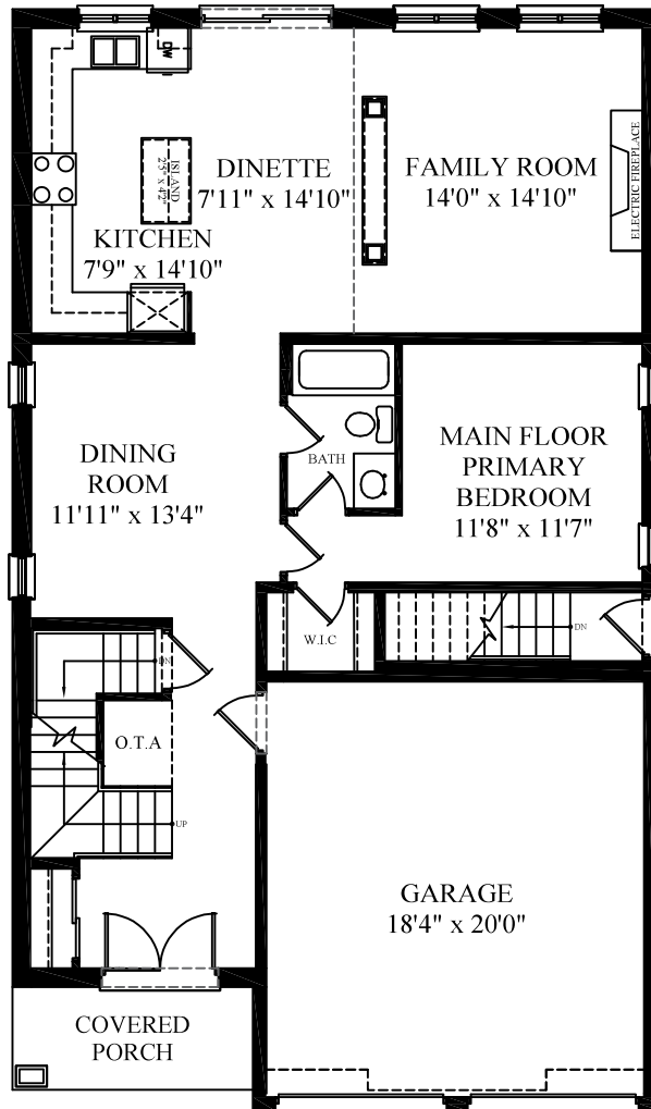
FIRST FLOOR PLAN 1,212 SQ. FT.
