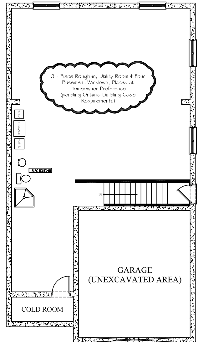
BASEMENT FLOOR PLAN 1,008 SQ. FT.
