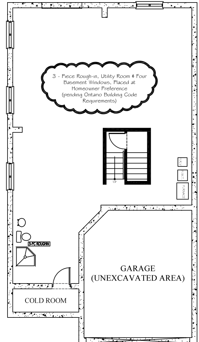
BASEMENT FLOOR PLAN 1,010 SQ. FT.
