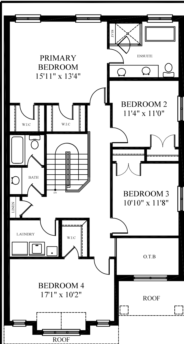
SECOND FLOOR PLAN 1,422 SQ. FT.
