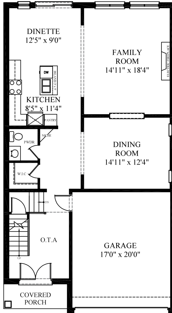
FIRST FLOOR PLAN 1,156 SQ. FT.
