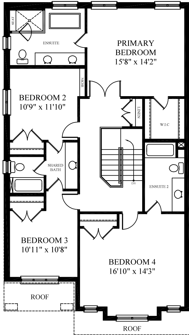
SECOND FLOOR PLAN 1,440 SQ. FT.
