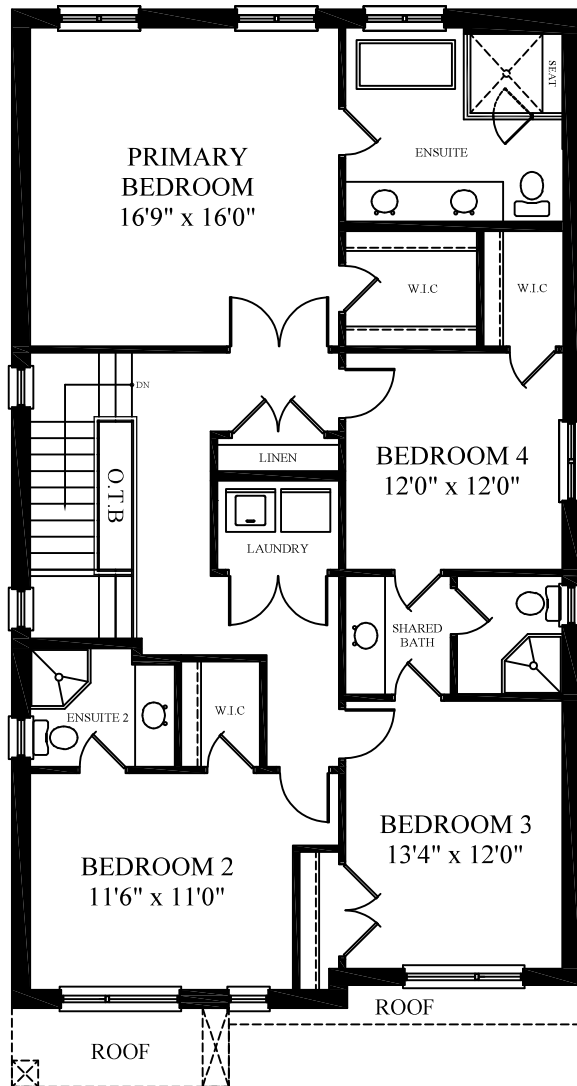
SECOND FLOOR PLAN 1,446 SQ. FT.
