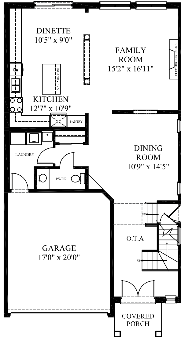
FIRST FLOOR PLAN 1,160 SQ. FT.
