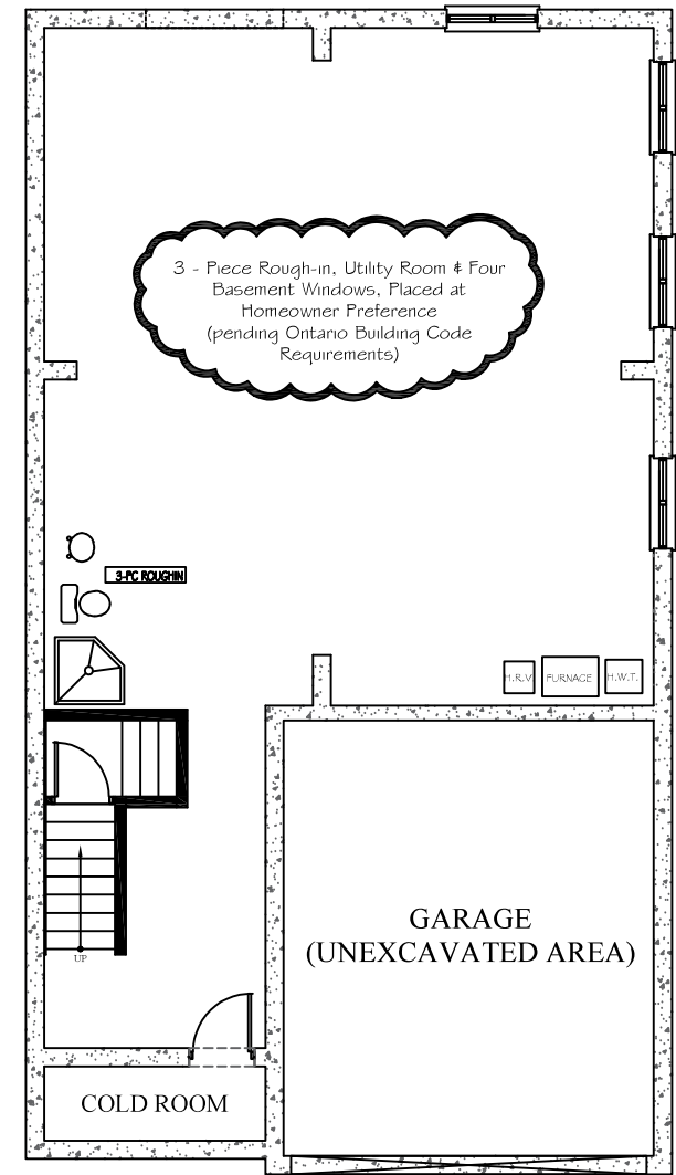
BASEMENT FLOOR PLAN 1,025 SQ. FT.
