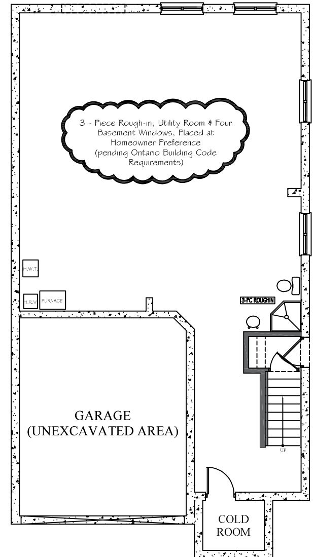
BASEMENT FLOOR PLAN 1,034 SQ. FT.
