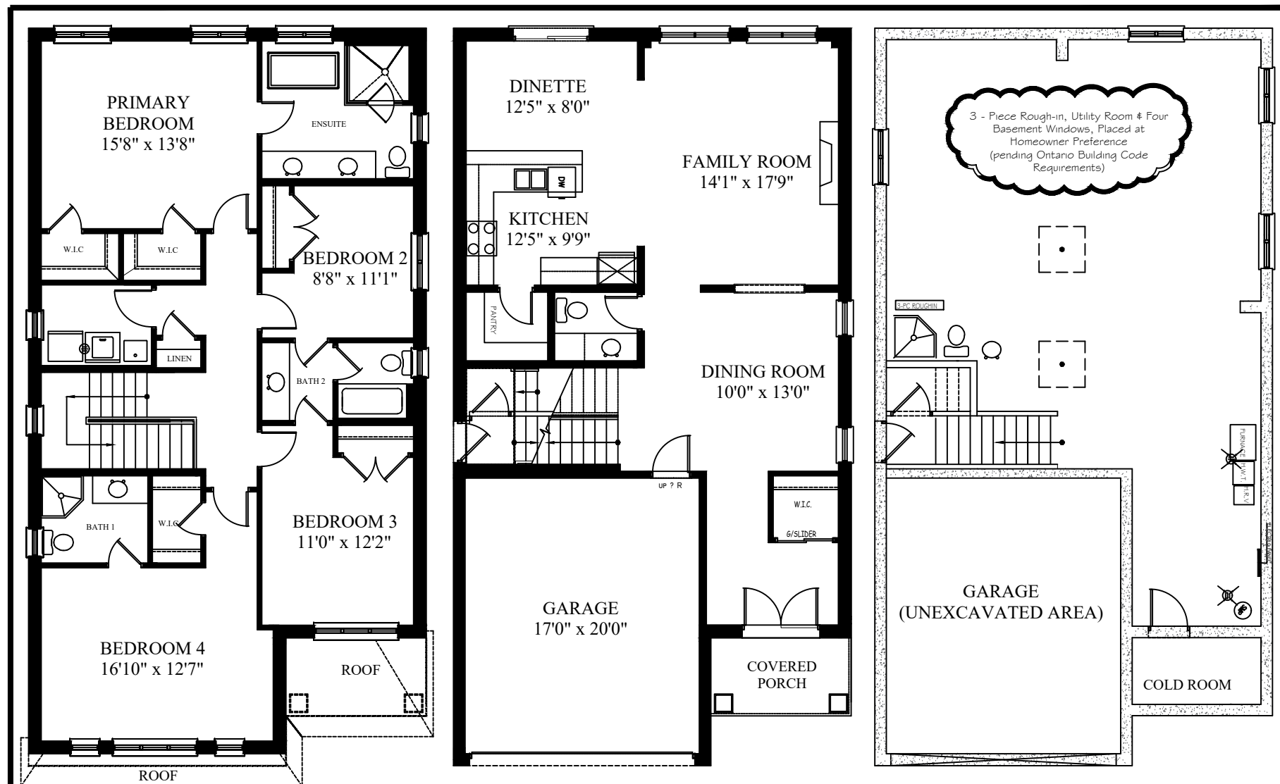
SECOND FLOOR PLAN 1,432 SQ. FT.
